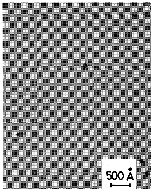
Fig. 1. Electron micrograph of colloidal palladium, Pd-PVP-MeOH/NaOH; original magnification, 100000 \times .
